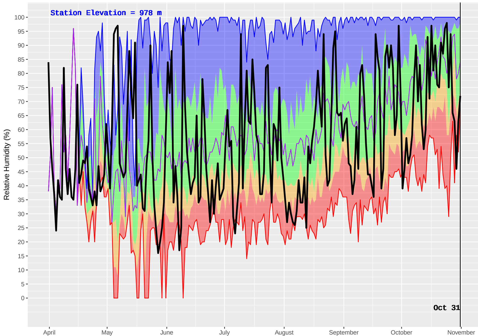
NILKITKWA (172) : Historical (1986–2016) and Current (2017) Noon Relative Humidity
