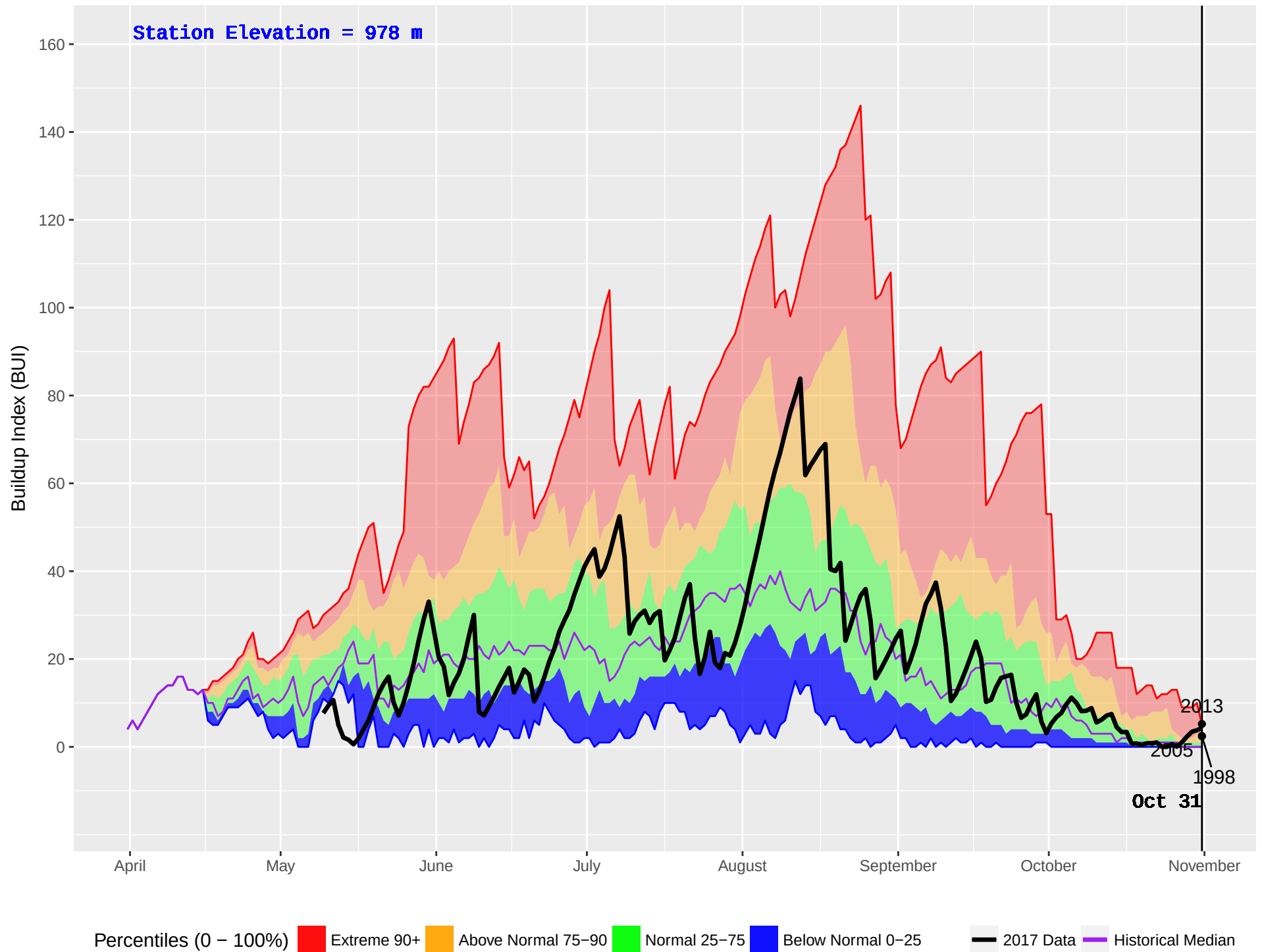
NILKITKWA (172) : Historical (1986–2016) and Current (2017) Noon Buildup Index (BUI)
